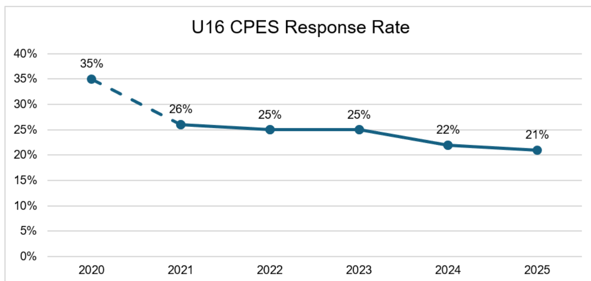
Figure 1: Adjusted response rates for U16 CPES
